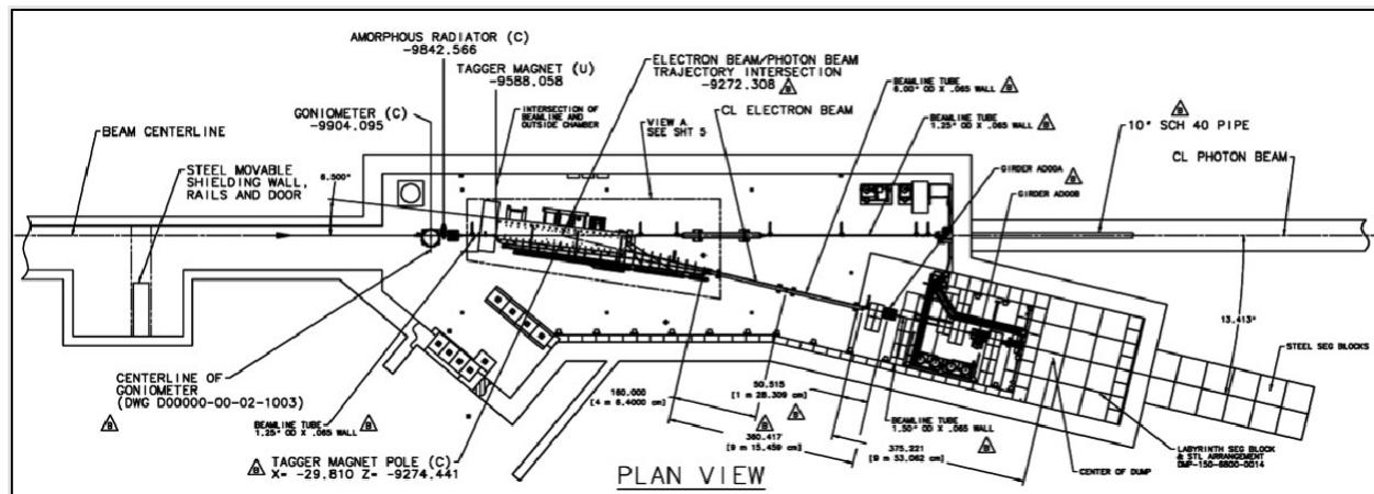
Figure 8. Hall D Tagger
