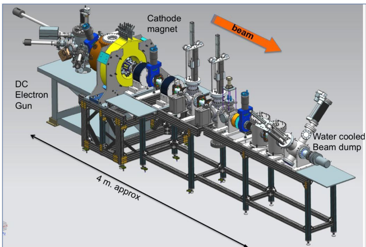
Figure 11. GTS Beamline
