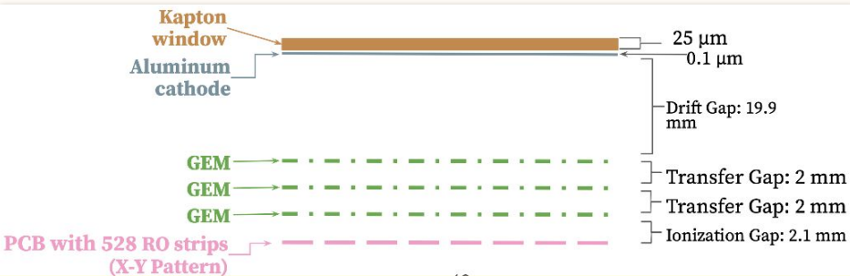
Triple-GEM TRD
