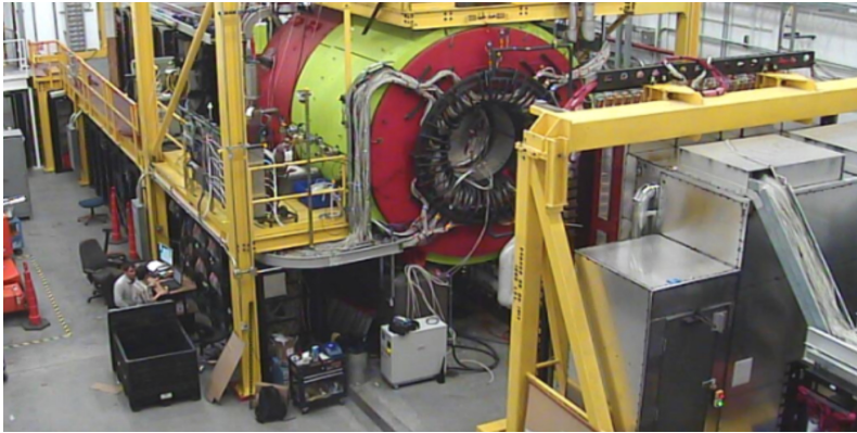
Hall D GlueX experiment – first to measure J/\psi at JLab (PRL 123, 072001 (2019))
