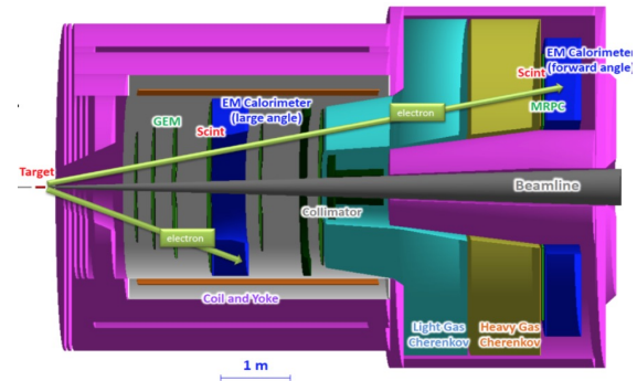
Hall A has SoLID E12-12-006 experiment approved to measure J/\psi via electroproduction and photoproduction
