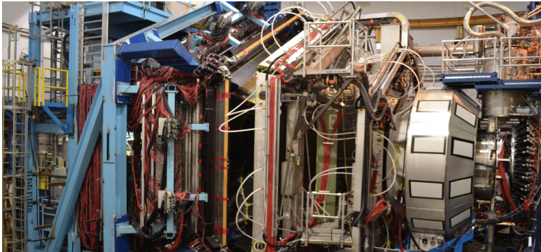
Hall B CLAS12 has experiments to measure TCS + J/\psi
