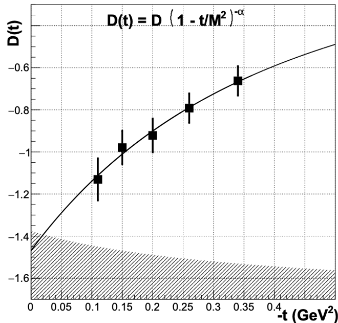
FIG. 2: The form factor D(t) as determined in the fit to the DVCS data. The hatched area represents the systematic uncertainties.
