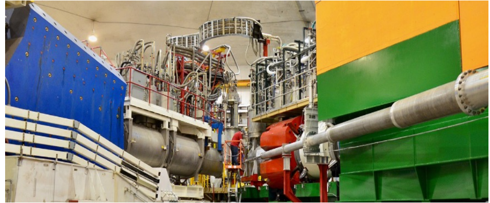
Hall C J/\psi 007 experiment - first to extract GFF and mass radius of proton (Nature 615 , pages 813–816 (2023))
