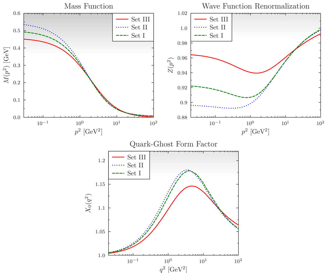
Figure 4. Mass function, M(p^2) , wave renormalization, Z(p^2) , and leading quark-ghost kernel form factor, X_0(q^2) , obtained with three sets of gluon and ghost propagators, \Gamma_\mu(k, p) = \Gamma_\mu^L(k, p) + \Gamma_\mu^T(k, p) and associated form factors of eqs. (2.44)–(2.55) in the DSE (2.15). Current-quark masses, strong couplings and renormalization scale as in figure 3.
