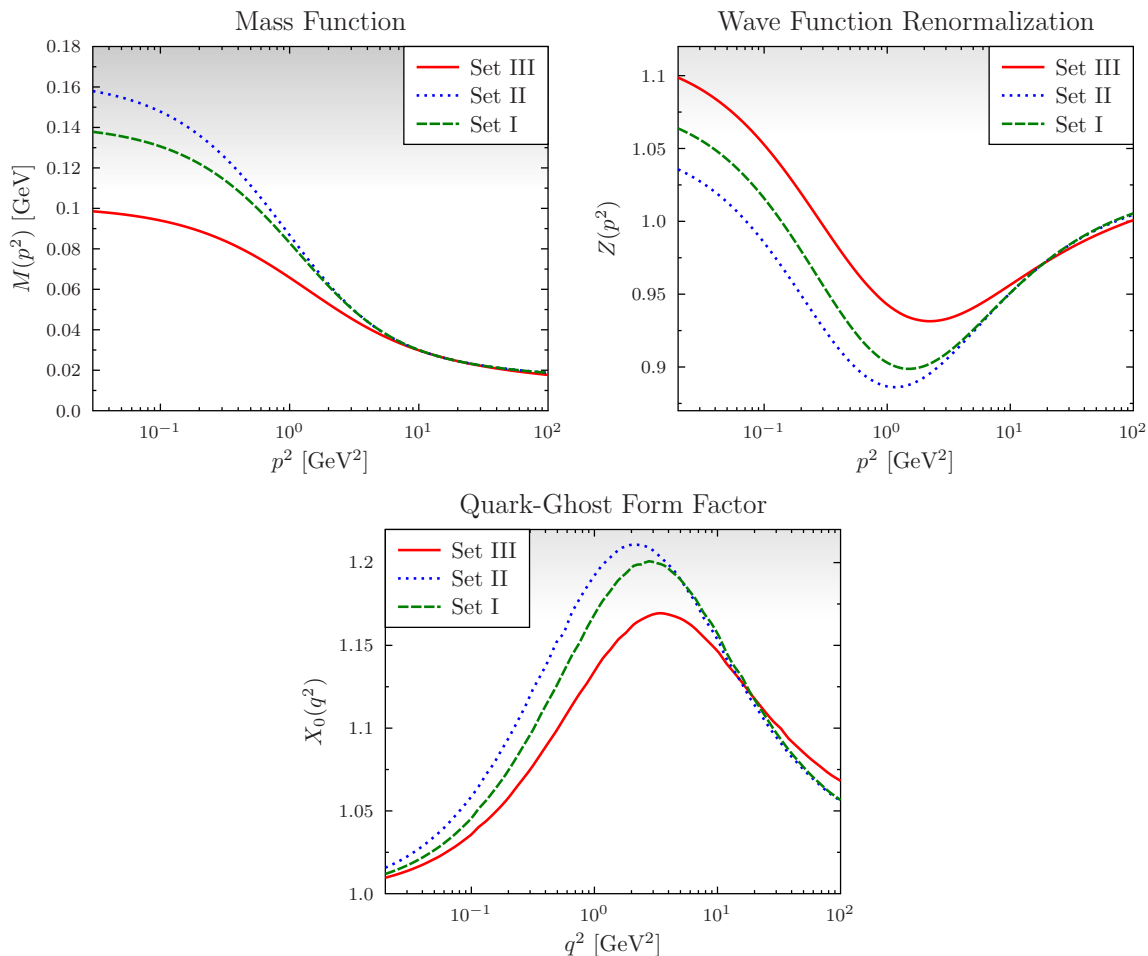
Figure 3. Mass function, M(p^2) , wave renormalization, Z(p^2) , and the quark-ghost kernel form factor, X_0(q^2) , for three sets of gluon and ghost propagators, using only \Gamma_\mu^L(k, p) and the form factors of eqs. (2.44)–(2.47) in the DSE (2.15). Set I [29] and II [35, 36]: \alpha_s(\mu) = 0.30 , m(\mu) = 25 MeV, \mu = 4.3 GeV. Set III [30]: \alpha_s(\mu) = 0.35 , m(\mu) = 25 MeV, \mu = 4.3 GeV.
