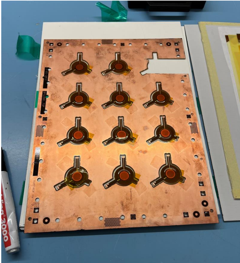
Batch of 8 single-channel uRWELL PCB
