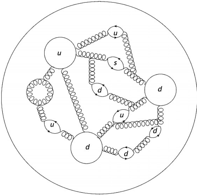
Neutron Composition
