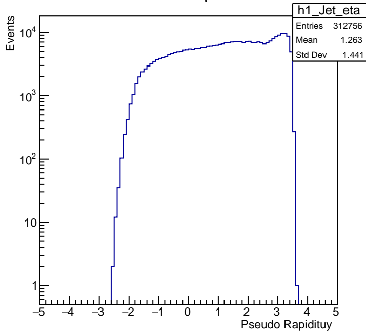
Jet \eta
