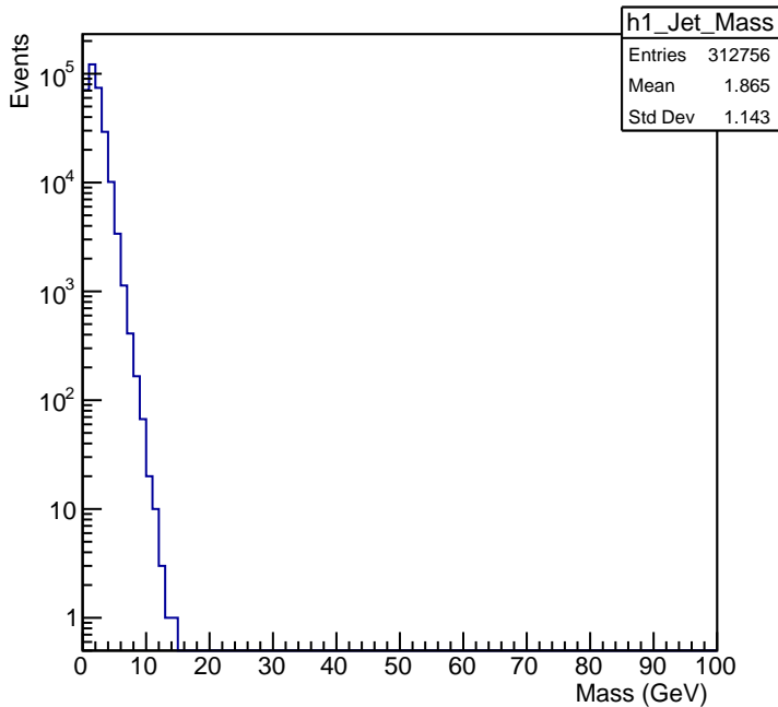
Jet Mass
