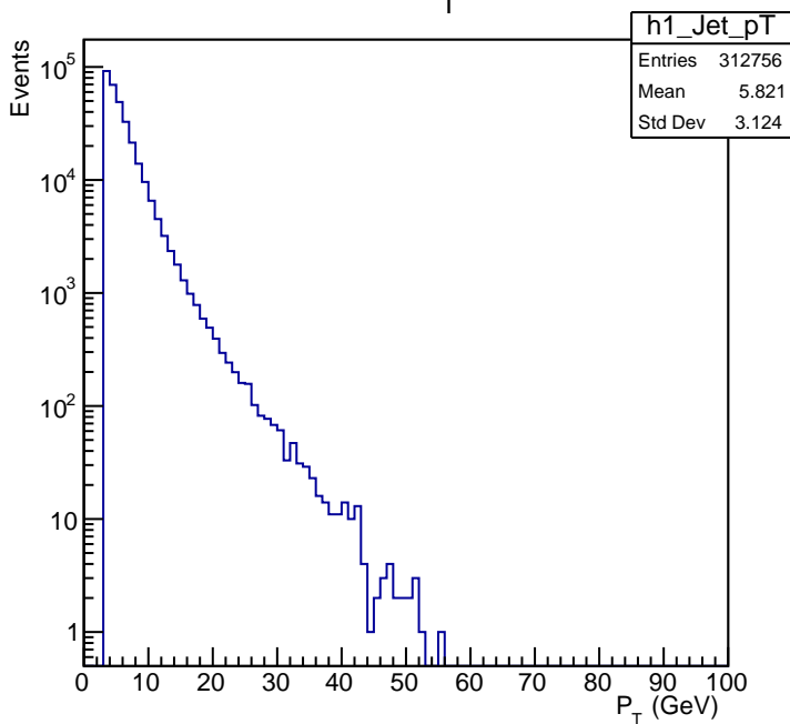
Jet P_T
