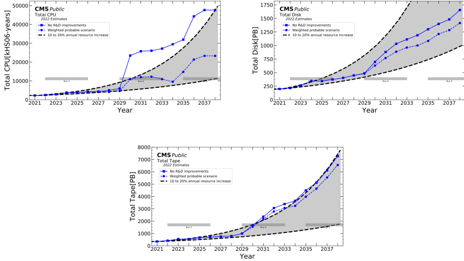
Figure 1. Estimated computing resource needs for CMS [10]. Shown are the modeled annual projections of total CPU and disk needs for CMS through Run 4. The estimated needs for each computing model scenario are shown by the blue lines. The gray band shows the projected resource availability for an example scenario that extrapolates the 2021 CMS pledged resources using an annual increase in available resources of between 10% and 20%. This assumes current WLCG cost projections [12] and a warranty + 3 years replacement cycle of hardware.
