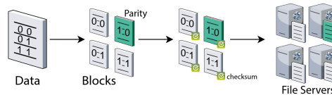
Figure 3: Erasure Coding in a Nutshell.
