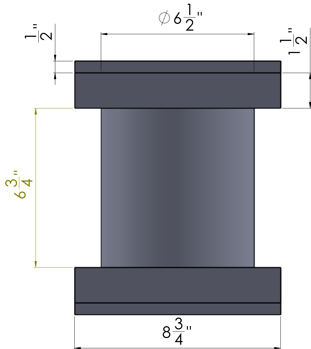
FOAM CAPS AND 5 LITER CAN SCALE 1:2
